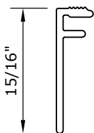
PAN-002 - 15/16" ALUMINUM JAMB EXTENDER FLASHING
