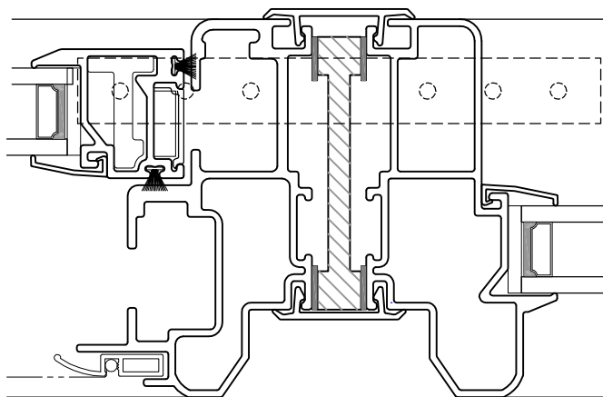
DOUBLE HUNG / 1001 PICTURE WINDOW
