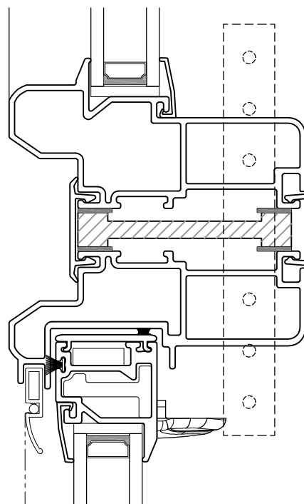
1001 TRANSOM / DOUBLE HUNG
