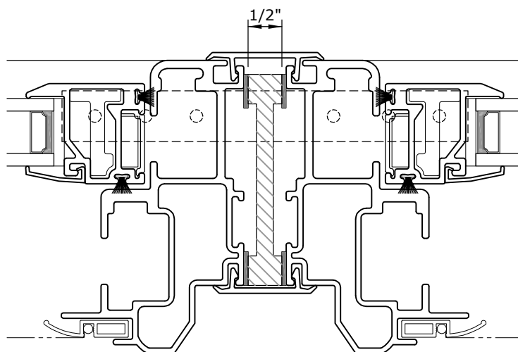
DOUBLE HUNG/DOUBLE HUNG
