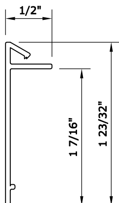
XF 12 - FLORIDA ( 1 \frac{7}{16} ") FLANGE
