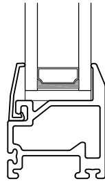
Standard Insul (1" to 1 1/8" O/A)
