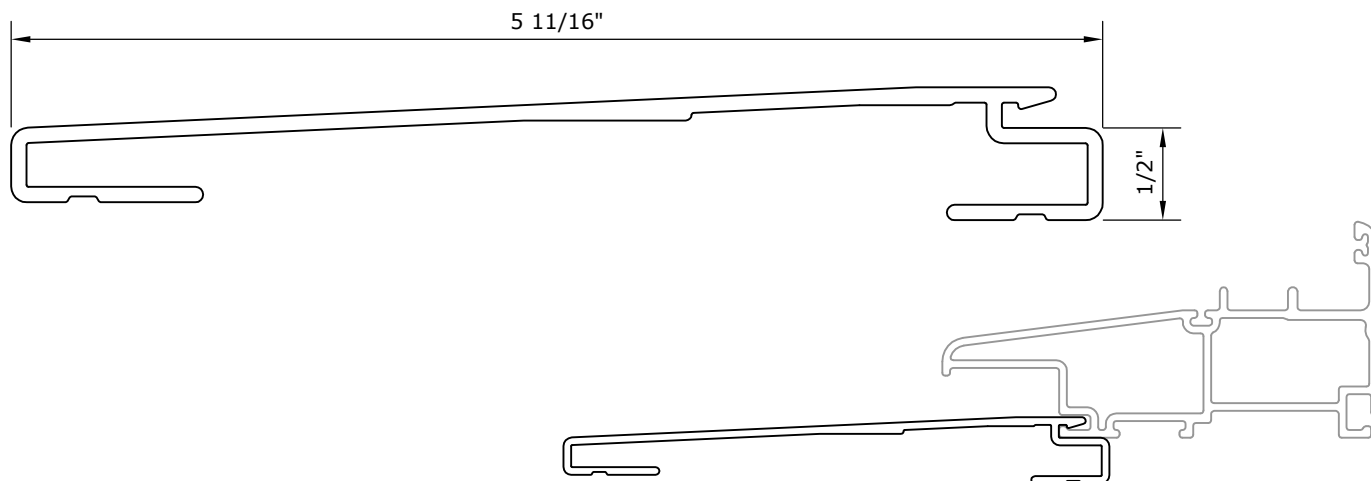
PAN-007 - 5" ALUMINUM EXTERIOR SLOPED SILL EXTENDER
