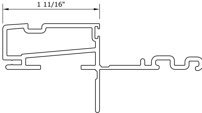
PAN-001 - 1 11/16" x 13/16" SQUARE NOSE ALUMINUM EXTERIOR SILL EXTENDER
