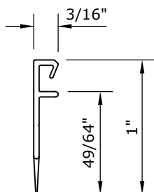
SV 38 - 3/4" SILL TRIM
