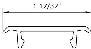
SS 54 - EXTERIOR ARCHITECTURAL MULLION COVER
